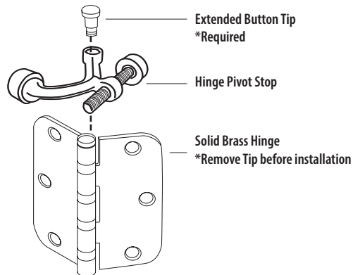
Hinge Pivot Stop for Solid Brass Hinge
