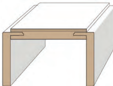
Sliding Door Jambs with Telescopic L-Shaped Casings. Extension is Optional.
