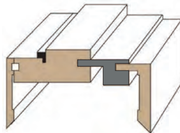
Jamb Extension to Accommodate Any Width of the Wall.
